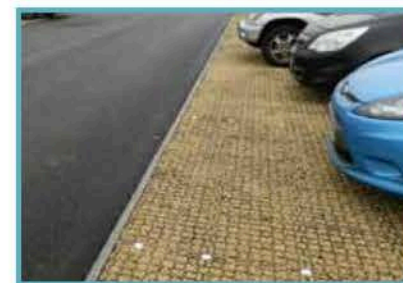
Plate 72 - Permeable parking
