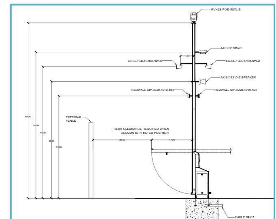
Plate 75 - Typical CCTV installation at an OnSS compound (source: National Grid)
