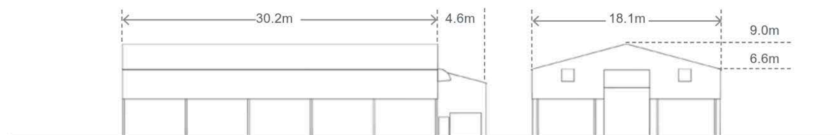
Plate 49 - Elevational study of barns at Holly Lodge Farm
