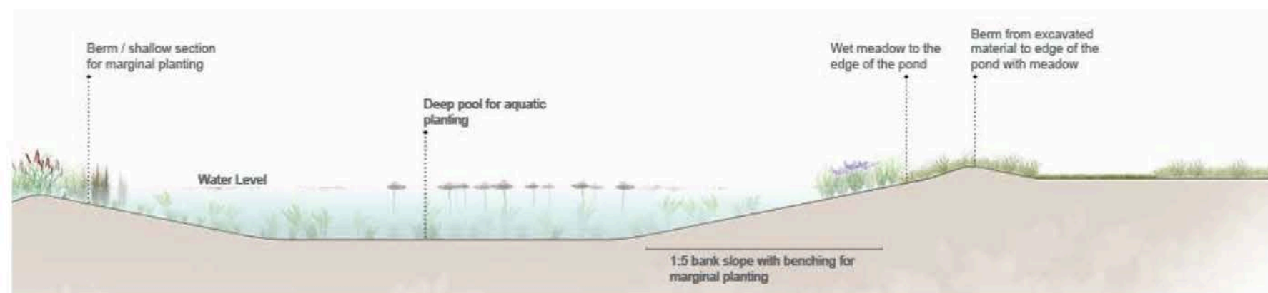
Plate 80 - Typical cross section through attenuation pond, designed for wildlife #2
