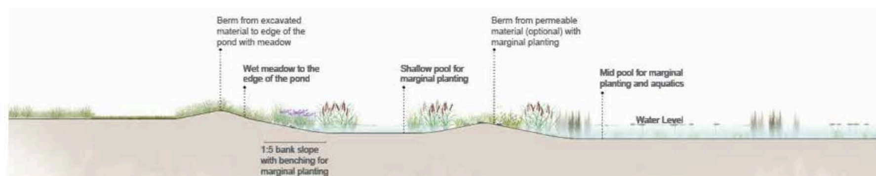
Plate 79 - Typical cross section through attenuation pond, designed for wildlife #1
