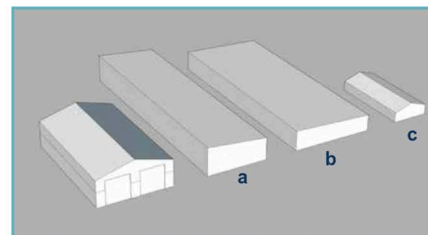
Plate 51 - Holly Lodge Farm 3D massing in comparison to a) STATCOM building, b) Control Building and c) Storage and amenity buildings
