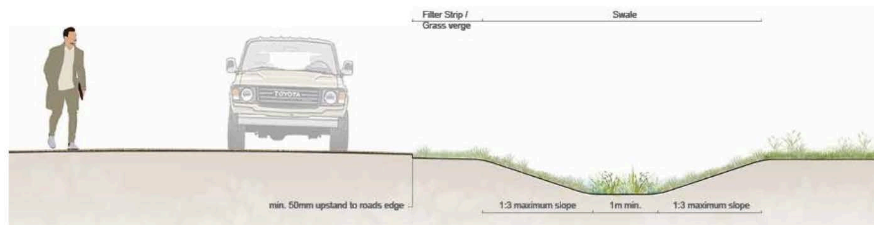
Plate 78 - Typical cross section through drainage swale
